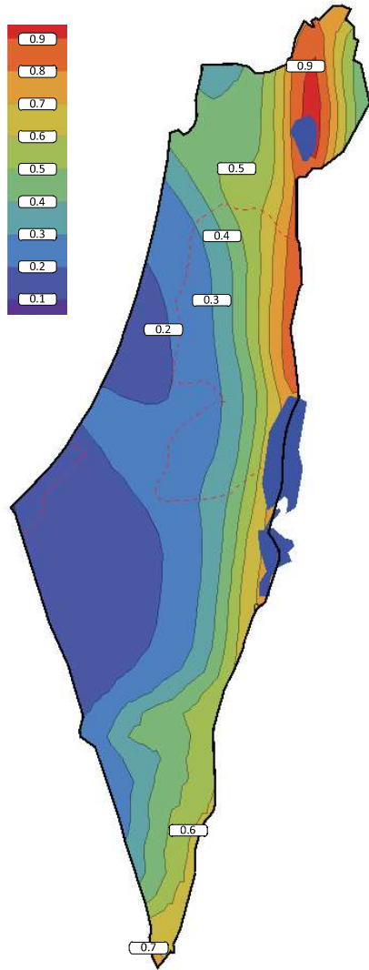
S_s 5%@50y
