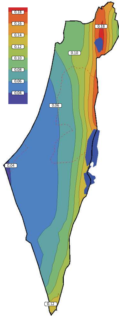
S_1 5%@50y
