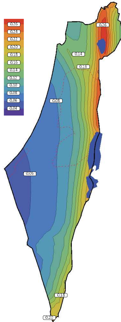
S_1 2%@50y
