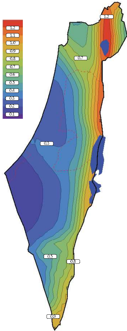
S_s 2%@50y
